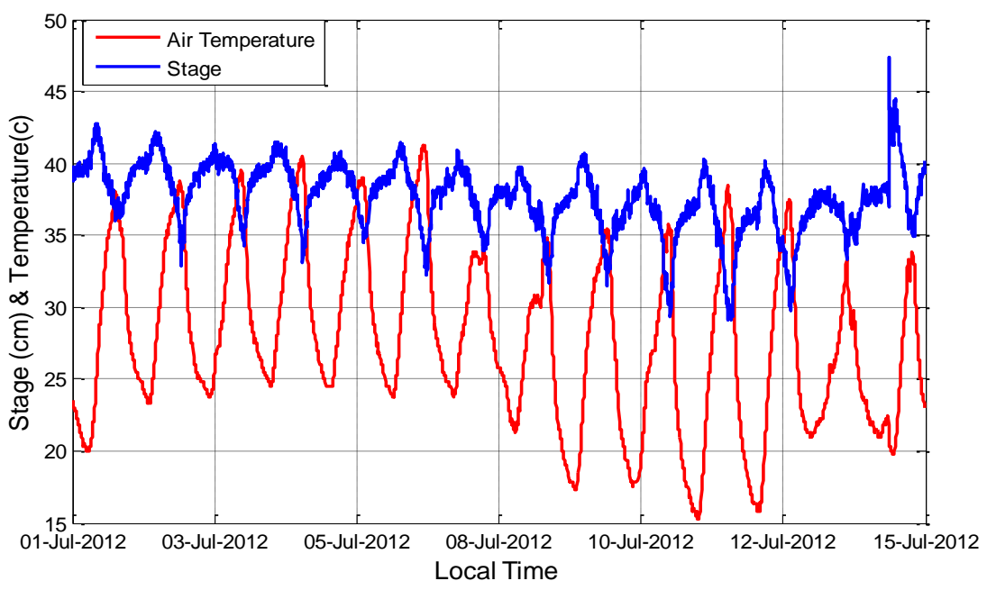
Figure 1.3: Stage and Temperature measured by USBS at Otter Creek (Station ID: OTTRCRK01).
