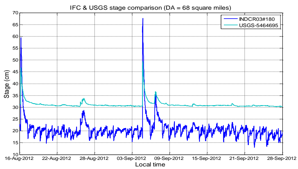
Figure 1.4: Comparison of stage measure by USBS (Station ID: INDCR03) and USGS gage (Station ID: 05464695) 3miles downstream at Indian Creek at Marion.
