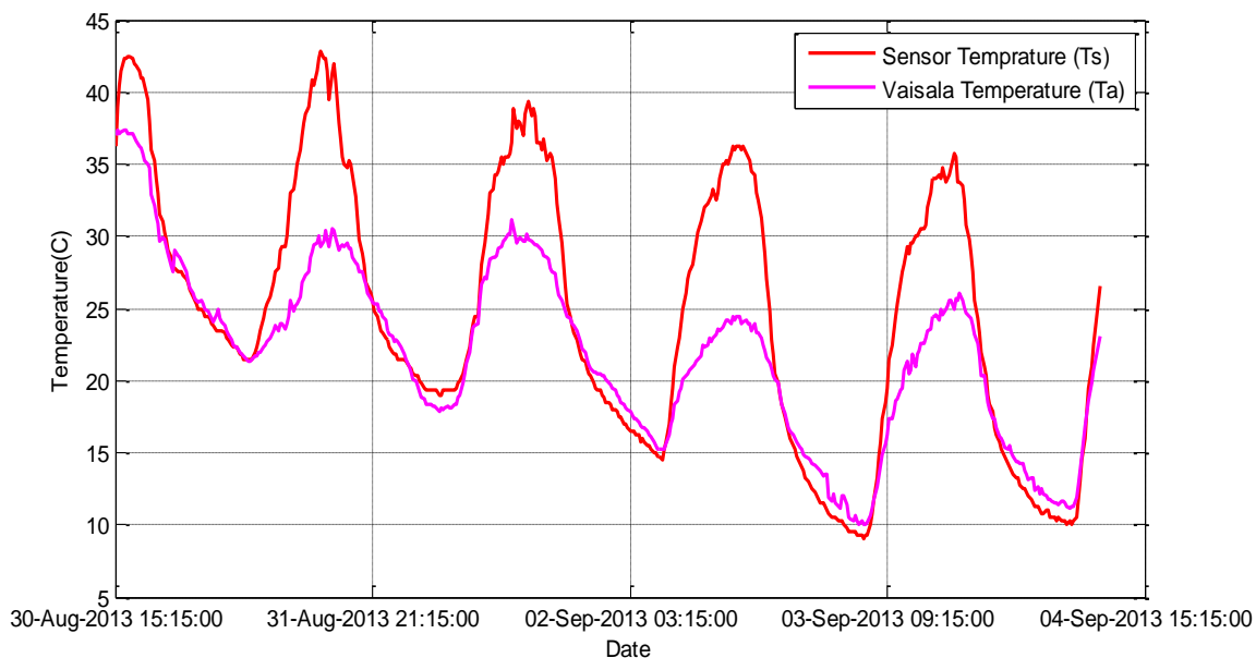
Figure 4.10: Temperature measured by Vaisala and USB internal temperature sensor
