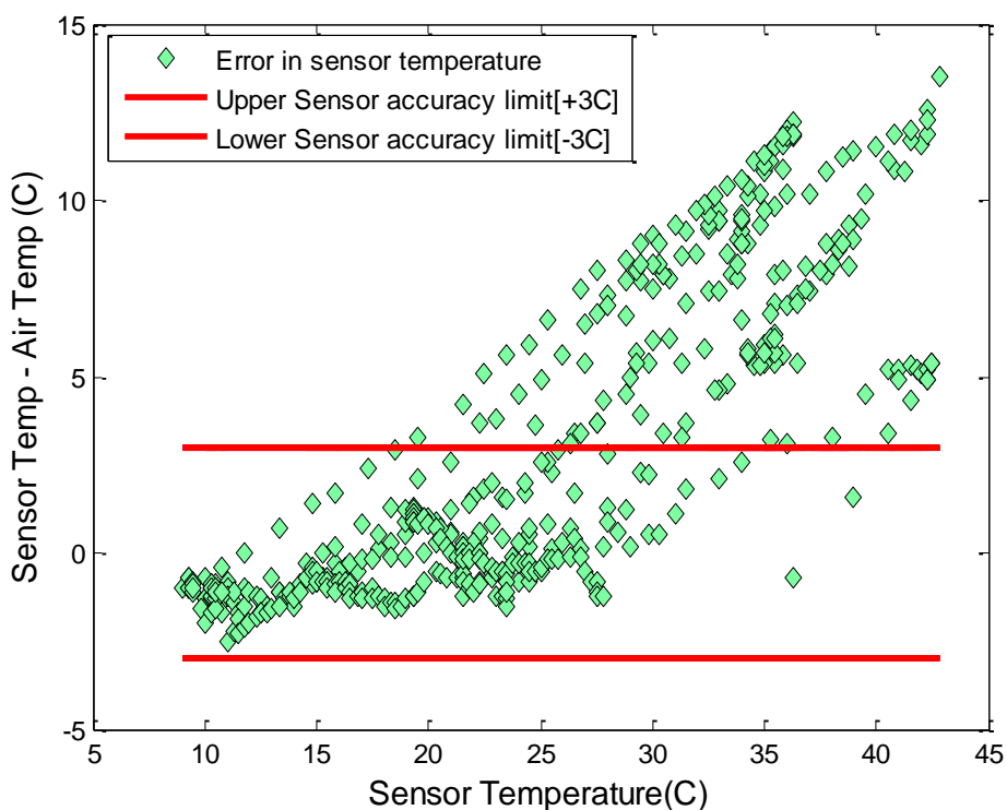
Figure 4.11: Scatter plot of temperature difference between USB internal temperature ( T_s ) and Vaisala air temperature ( T_a ). Red line indicates upper and lower USB internal temperature accuracy.
